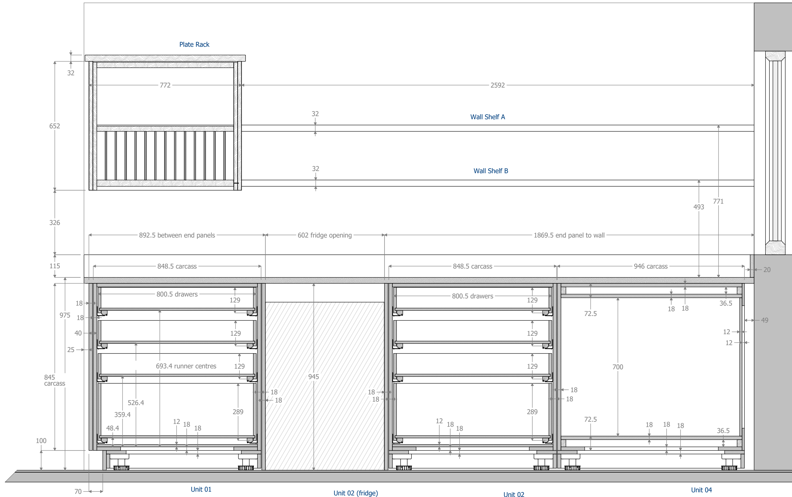
Section Through Fridge Run
